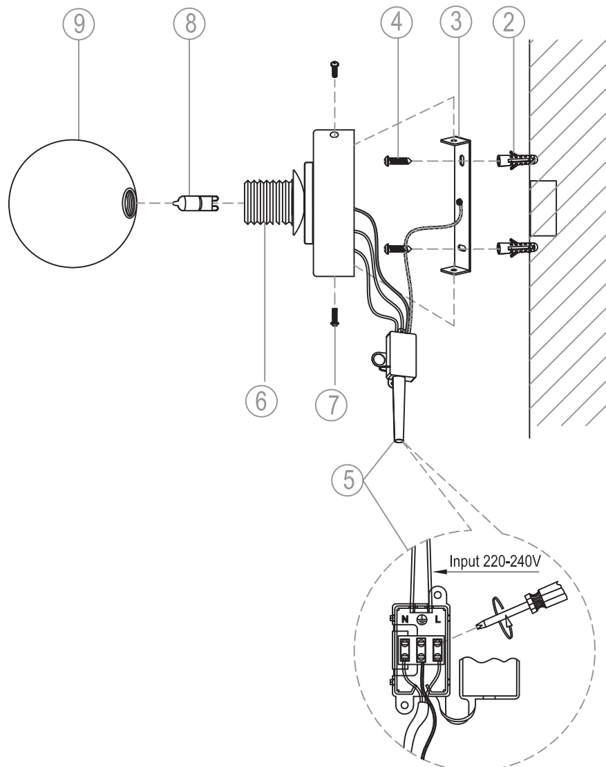
wire connection
