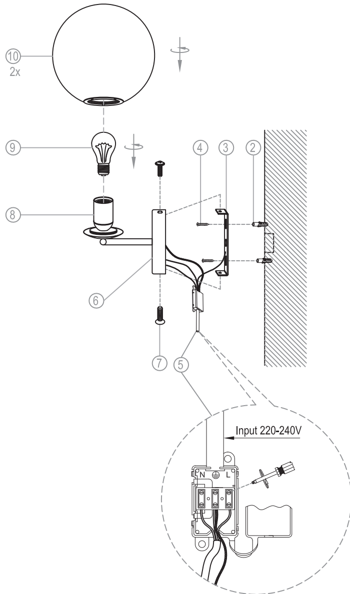
wire connection
